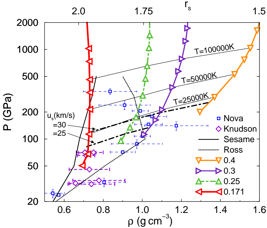
Figure 2. Pressure density diagram showing Hugoniot measurements [1, 2, 3] and results from chemical model calculations [4, 5] starting from the uncompressed liquid deuterium state ( \rho_0 = 0.171 \text{ g cm}^{-3} ). The triangles indicate Hugoniot curves from PIMC simulations for different initial densities \rho_0 given in the legend in units of \text{g cm}^{-3} . The thin solid lines are isotherms, the dash-dotted lines represent final shock states generated with the same shock velocity ( u_s = 25 and 30 \text{ km/s} ) starting from different initial compressions.
