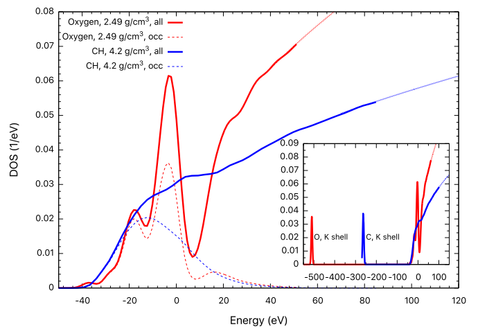
FIG. 4. Density of state of polystyrene in comparison with that of oxygen at 10^5 K. The dashed curves denote the occupied states, and the dotted lines are extrapolations of the free-electron density of state. The Fermi energies are aligned at E=0 eV.
