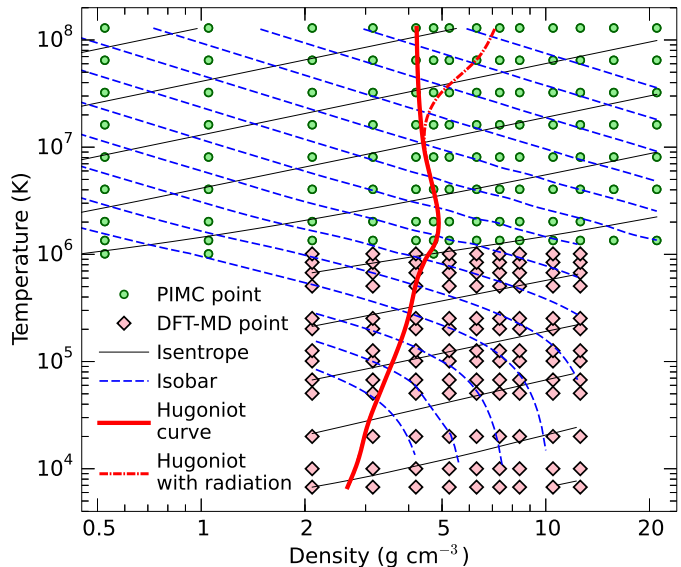
FIG. 1. Temperature-density profile of the principal Hugoniot curve of polystyrene CH (initial density \rho_0=1.05 g cm -3 ) with and without radiation correction, obtained from the equation of state calculated in this work. Isobar and isentrope profiles are co-plotted. The symbols mark the simulation conditions.
