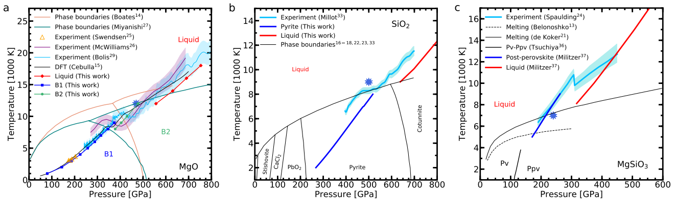
FIG. 1. Hugoniot curves and phase diagram of silicates. Phase diagram of (a) MgO [14, 27], (b) SiO 2 [16–18, 22, 23, 33] and (c) MgSiO 3 [20, 21, 36] are plotted. We added our predictions for the Hugoniot curves in the different phases as well as other first-principles predictions [15, 37] and experimental shock results [25, 26, 33, 34]. The shaded areas represent the experimental uncertainty. The blue stars indicate the P - T conditions we chose for the liquid/solid comparison.
