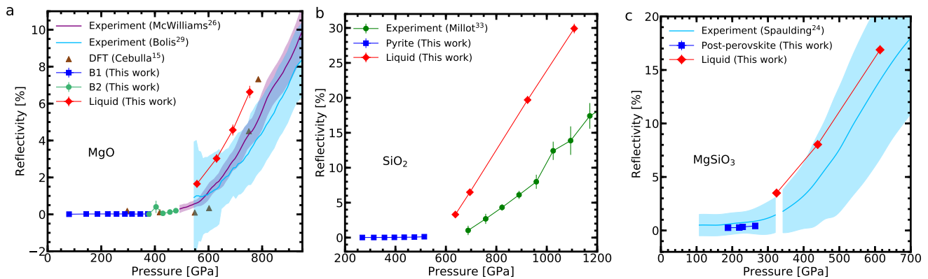
FIG. 4. 532 nm reflectivity along the principal Hugoniot. We plotted our calculated reflectivity (with a one- \sigma errorbar) in the different phases of (a) MgO, (b) SiO 2 and (c) MgSiO 3 along their respective Hugoniot curves as described in Fig. 1. We added previous numerical results for MgO [15], and systematically compared with available experimental results [26, 28, 33, 34] including their uncertainty.
