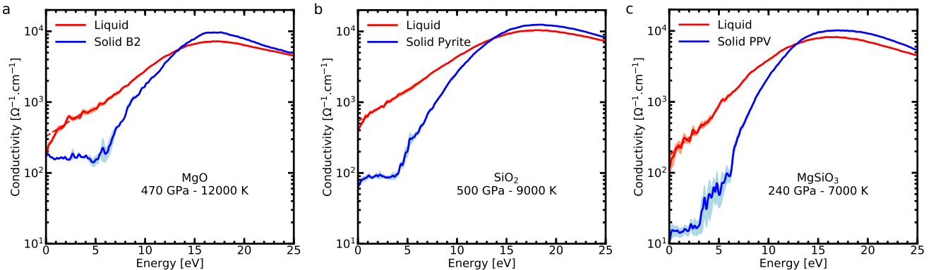
FIG. 3. Electric conductivity. The liquid (red) and the solid (blue) electric conductivities as a function of the excitation energy are plotted for (a) MgO, (b) SiO 2 and (c) MgSiO 3 . The conditions are the same as those of Fig. 2. The shaded region is an indication of the one-sigma statistical uncertainty. We plotted in dashed lines the extrapolation of the conductivity in the liquid phase towards the direct current (DC) value (see the Method section).
