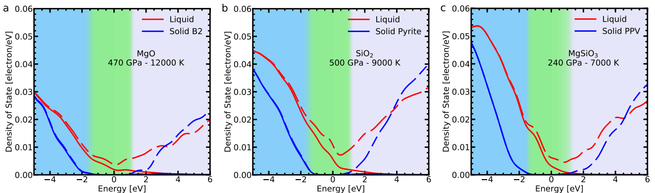
FIG. 2. Electronic density of states (DOS) of silicates. The liquid (red) and the solid (blue) DOSs with the Fermi level shifted to 0 eV are plotted for (a) MgO, (b) SiO 2 and (c) MgSiO 3 . The dash-dotted lines are the complete DOSs and the full the occupied DOSs only. The conditions were chosen so that they are close to the respective Hugoniot curve [26, 33, 34] and the expected phase boundary [20, 27, 33] as shown by the blue stars on Fig. 1. The blue shaded region represents the valence band in the solid, the green one is the gap and the light purple one is the conduction band.
